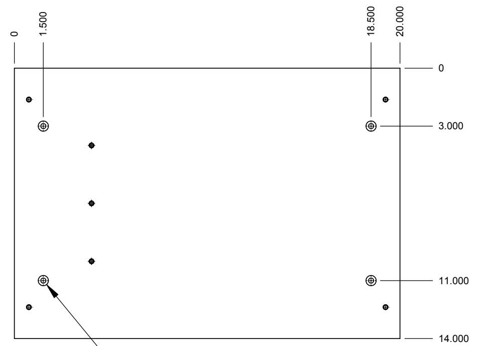
4X \phi .266 THRU ALL \surd \phi .531 X 82° Mounting Pattern Use 1/4 Countersunk Screws for Mounting
